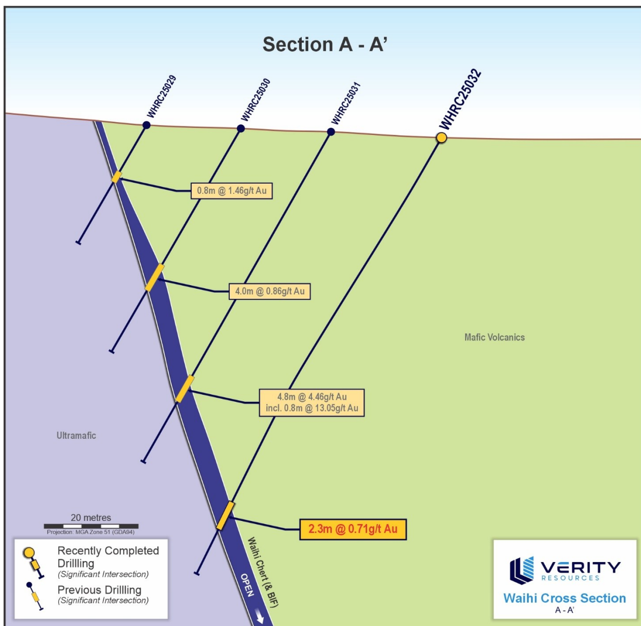
Figure 2. Representative cross section A-A' through the core of the Waihi mineralisation showing the BIF main mineralised lode.
