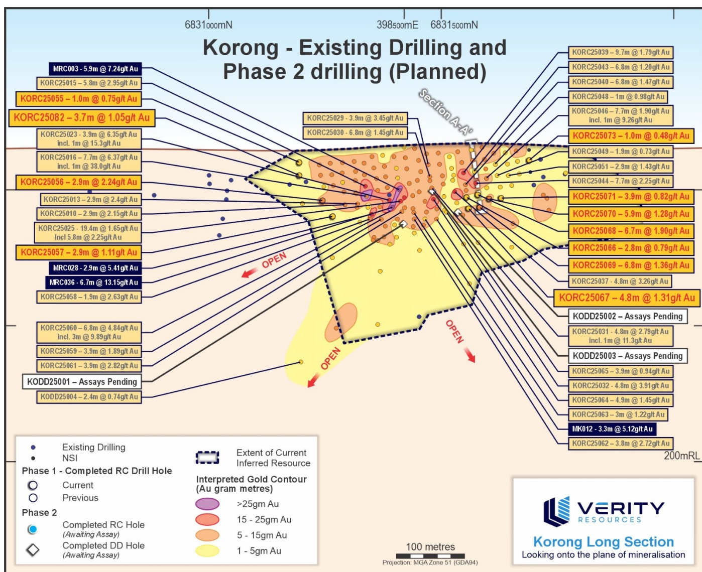
Figure 3. Long Section view of recently completed drilling with assays, looking from the hanging wall down onto plane of mineralisation. Outline of the current 154koz Au Inferred Resource is shown (black).
