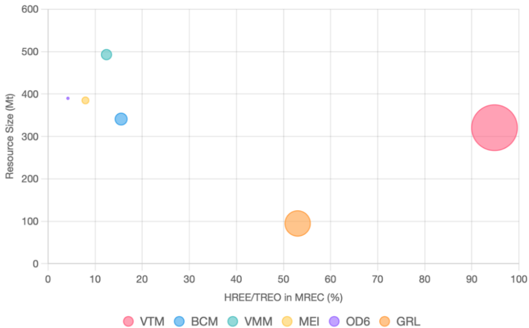
Figure 3: Bubble size represents Terbium (Tb) percentage in Mineral Resource Estimate (MREC) Total Rare Earth Oxide (TREO); horizontal axis shows Heavy Rare Earth Elements (HREE) to TREO ratio (%); vertical axis shows resource size (Million tonnes, Mt), comparing Victory Metals initial MREC with MREC data for peer entities.
