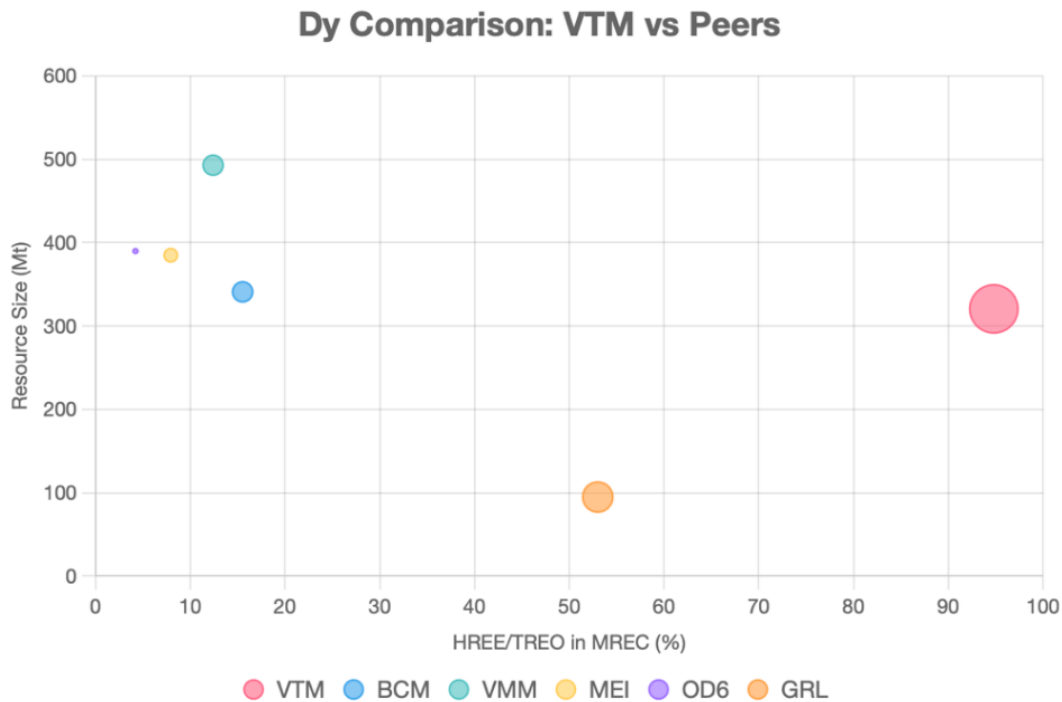
Figure 2: Bubble size represents Dysprosium (Dy) percentage in Mineral Resource Estimate (MREC) Total Rare Earth Oxide (TREO); horizontal axis shows Heavy Rare Earth Elements (HREE) to TREO ratio (%); vertical axis shows resource size (Million tonnes, Mt) comparing Victory Metals initial MREC with MREC data for peer entities.
