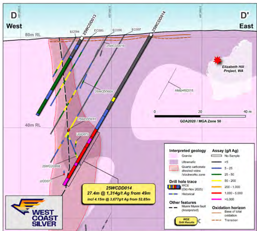
Figure 5. Cross Section showing silver mineralisation in 25WCDD014
