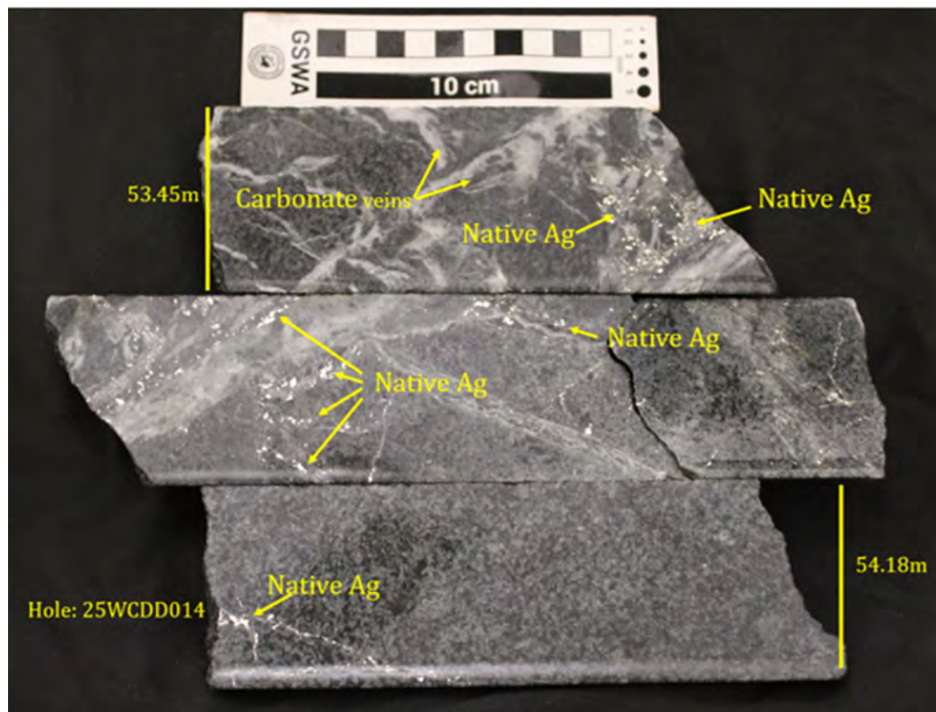
Figure 6. Photograph of cut half HQ3 drill core (25WCDD014) from 53.45m to 54.18m showing 2mm to 4mm grains of native silver hosted within and adjacent to 1cm to 3cm thick carbonate veins in an ultramafic host rock.
