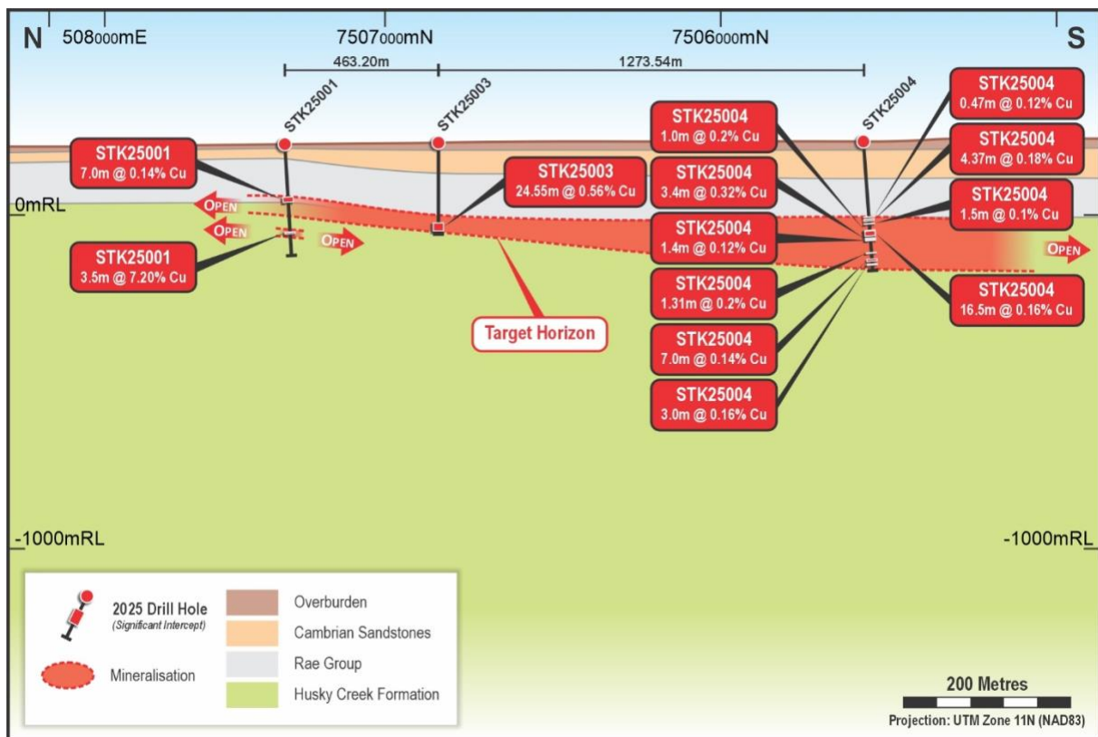
Figure 2 - Section of drillholes STK25001 to STK25004, which defines 1.7km strike length of copper mineralisation focussed on the contact of the Rae Group and Husky Creek Formation.
