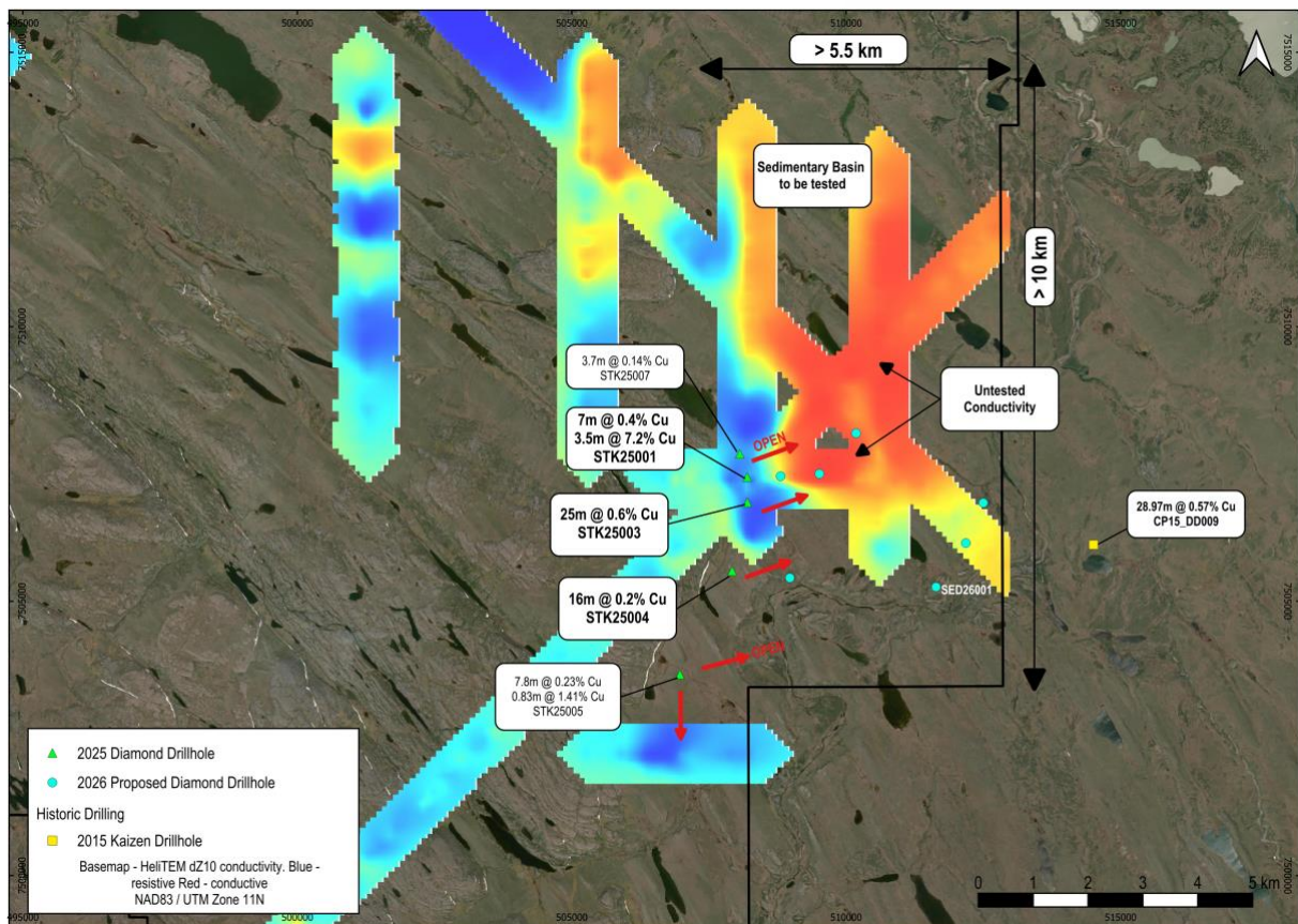
Figure 1 - Map of planned drilling at Rae Group Eastern Sedimentary Targets, overlaid with 2025 drillholes and airborne EM conductivity response flown in 2025. The map shows an area of untested conductivity to the east. Drillhole STK25001 which returned 7m @ 0.41% Cu from 177m within the sediments of the lower Rae Group sits on the western edge of the conductivity anomaly.
