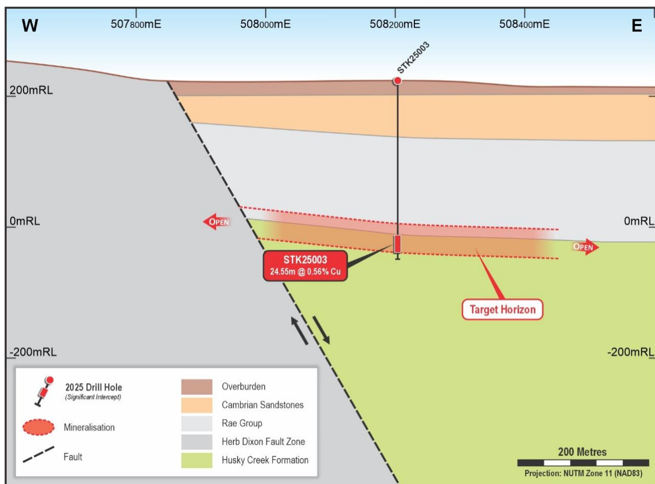
Figure 3 - Section of drillhole STK25003 highlighting the 24.55m interval of 0.56% Cu that was intercepted immediately below the redox boundary contact.
