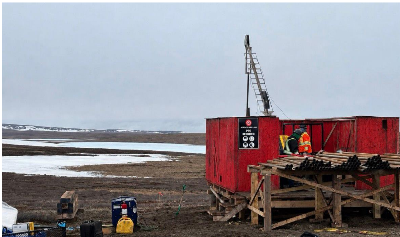
Figure 4 - Photograph of diamond drilling rig positioned over SED26001.
