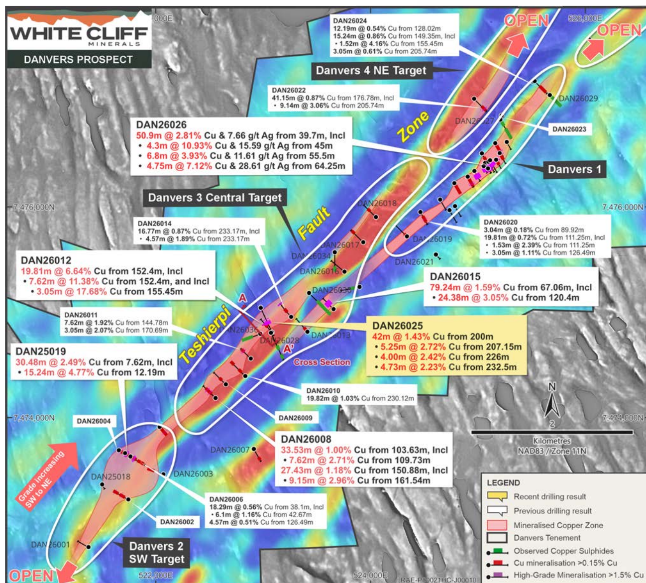
Figure 1 - Map of 2026 drillholes in the Teshierpi Fault Zone. Basemap of EM anomaly (X component) from 2025 geophysical survey. Interpreted mineralisation trend highlighted by white outline between the observed downhole intervals of copper sulphides.
