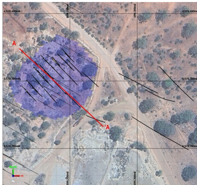
Figure 3: Repeater plan view with section line A-A
