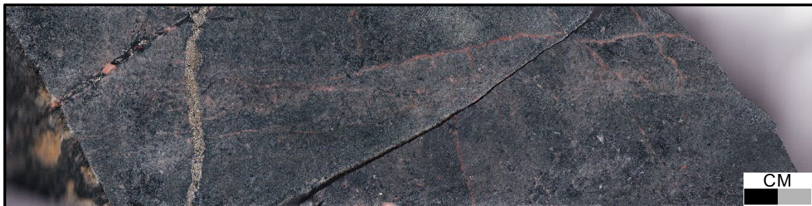
Figure 8: SPD034 362.7m 5.07 g/t Au . Pyrite-carbonate-chlorite vein overprinting chlorite-k-feldspar-pyrite vein in andesite.
