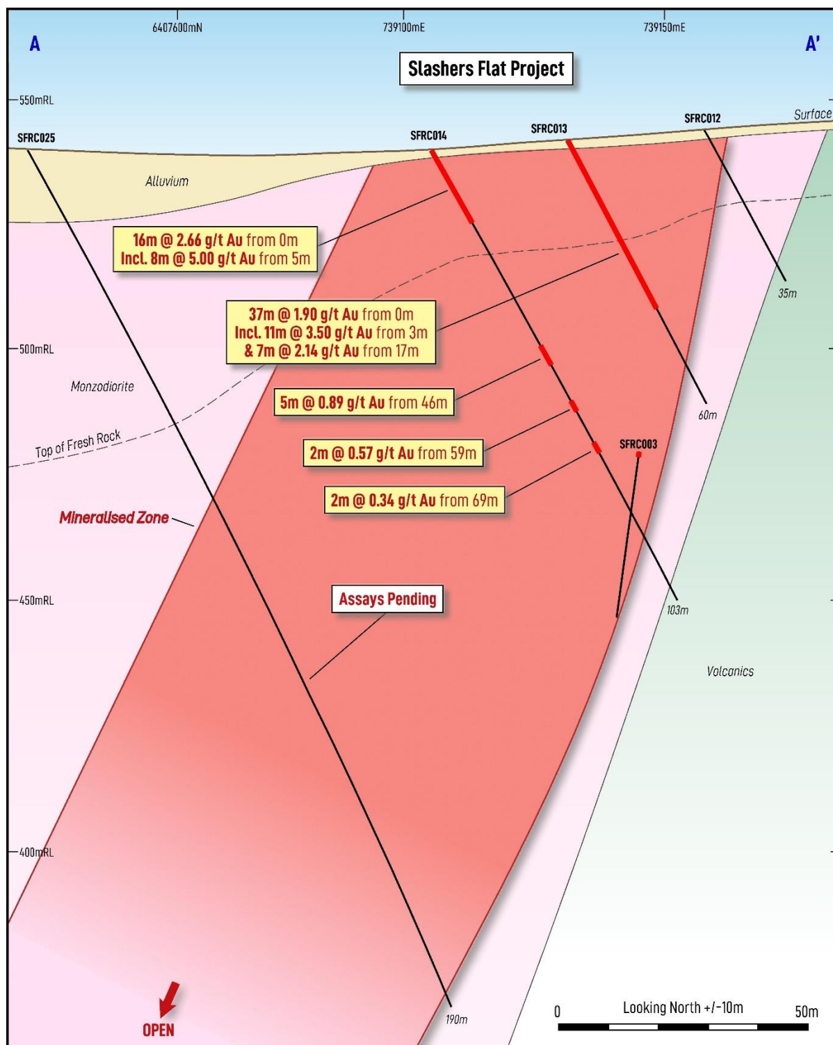
Figure 2: Cross-section showing broad gold mineralisation in holes SFRC012, SFRC013 and SFRC014. The mineralised zone remains open at depth.
