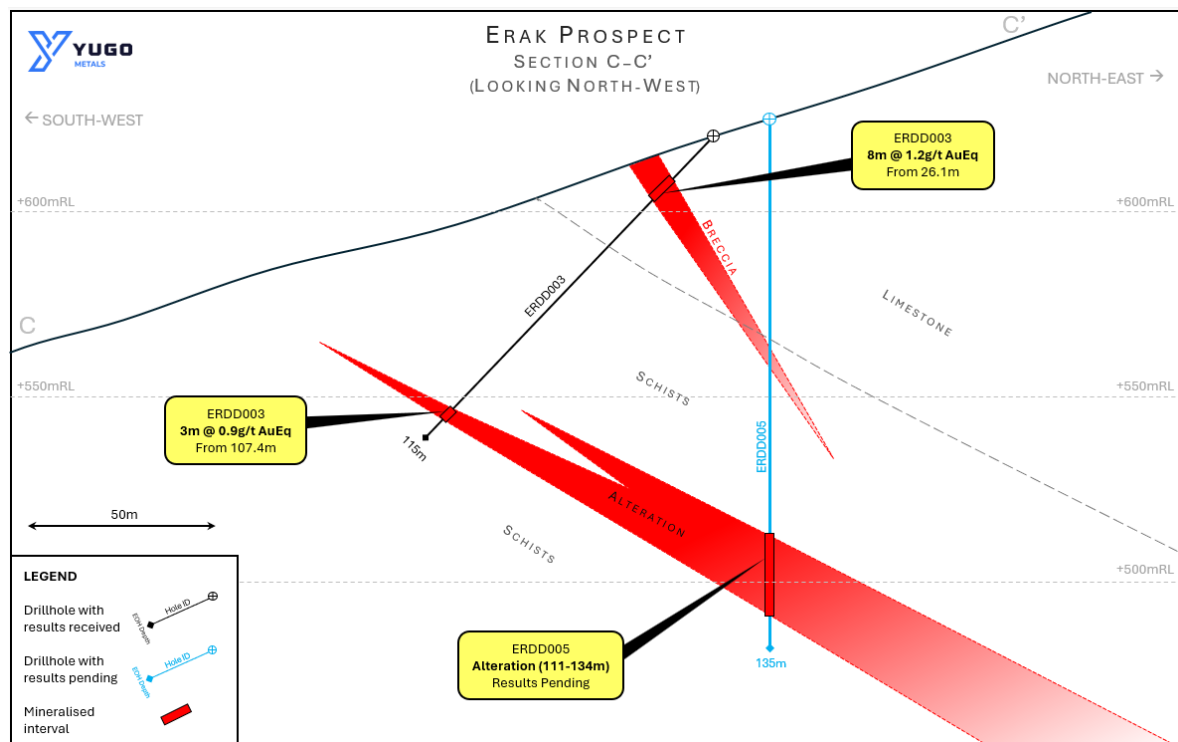
Figure 5: Erak Prospect (Sinjakovo Project), drilling cross-section C-C'
