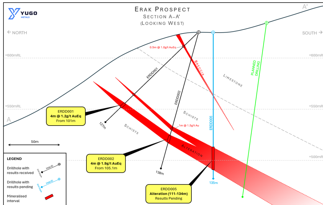
Figure 3: Erak Prospect (Sinjakovo Project), drilling cross-section A-A'
