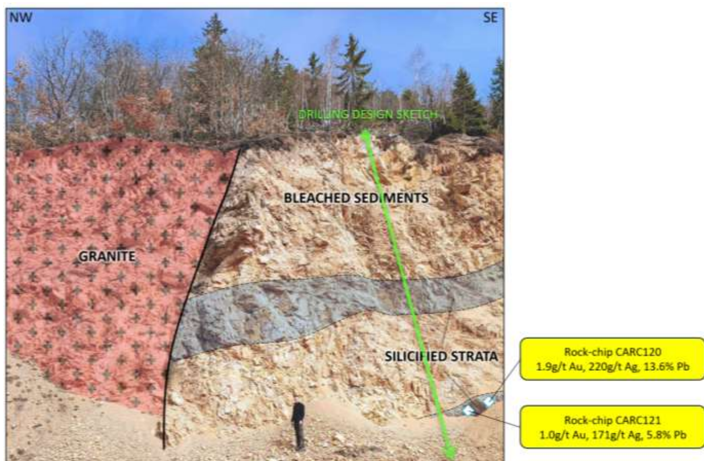
Figure 5: Cajnice Project, Majdan Au-Ag-Pb Prospect, photo of cliff profile
