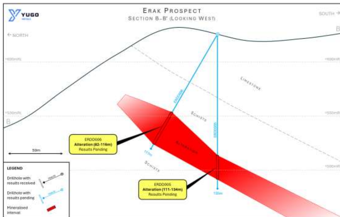
Figure 3: Erak Prospect (Sinjakovo Project), drilling cross-section B-B'
