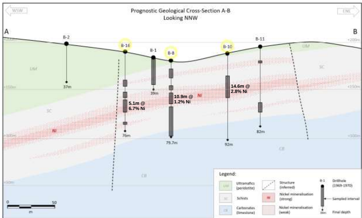
Figure 7: Sockovac (Petrovo) cross-section showing historical drill holes with interpreted geology
