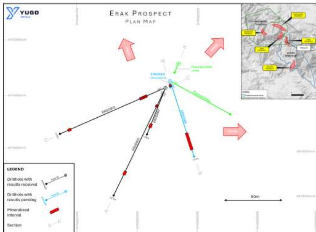
Figure 1 Erak Prospect (Sinjakovo Project), plan map showing drilling program
