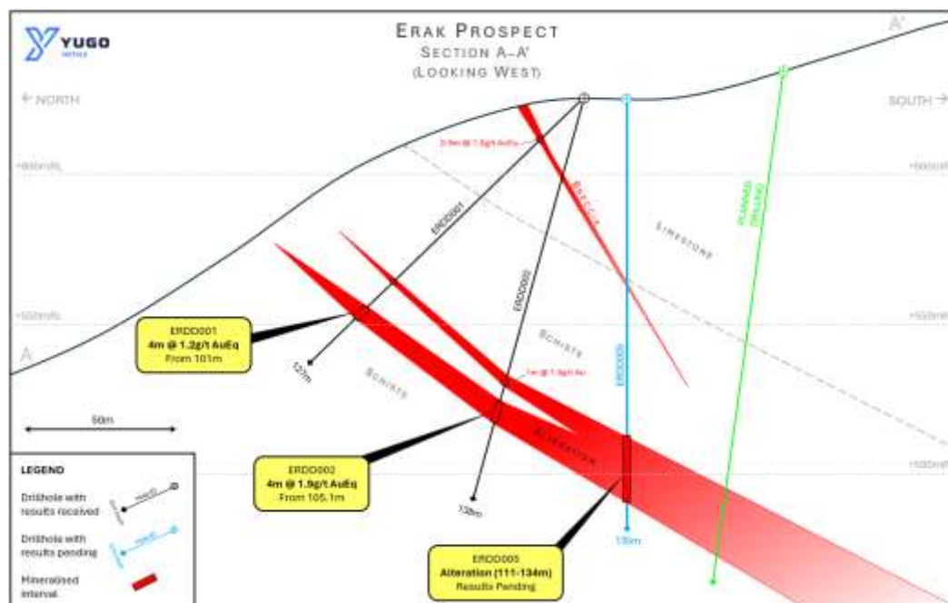
Figure 2: Erak Prospect (Sinjakovo Project), drilling cross-section A-A'
